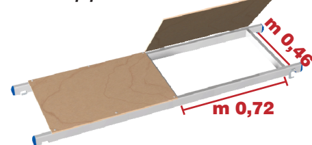
Piano di lavoro con botola Piano in resinato antiscivolo. Work platform with trapdoor in anti-slip phenolic resin film.
